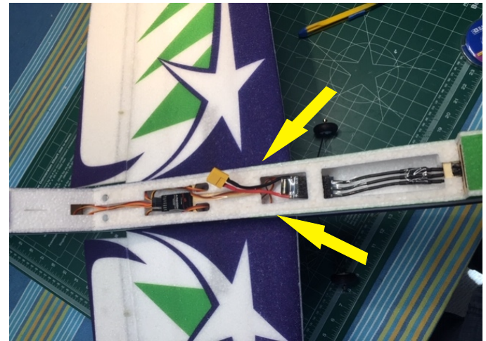
15 Install Servo, Aileron, Control Horn and Servo Linkage to other Wing as in Step 12 Medium CA Wing
