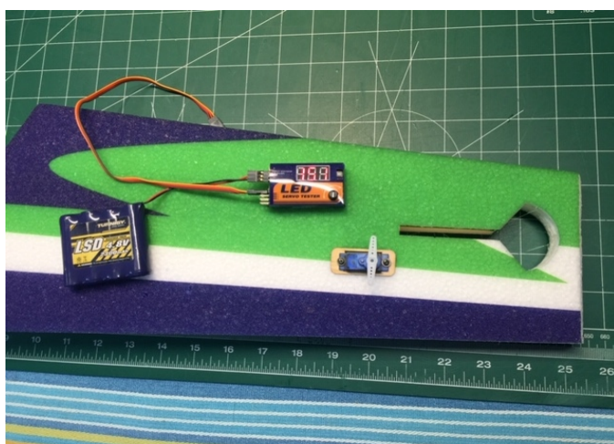
4 Install the Elevator and Rudder Servos with the Hub closer to the Back of the Plane. Center them electronically with Servo Tool or Your Receiver/Transmitter Combo.
