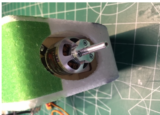
5 Install Motor using 4 Supplied Screws
