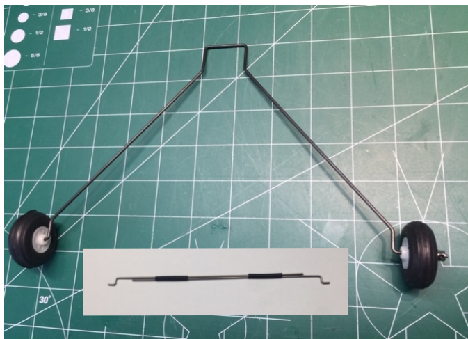
6 Assemble Landing Gear, and Prepare Servo Linkages with supplied heat shrink but don't shrink yet.
